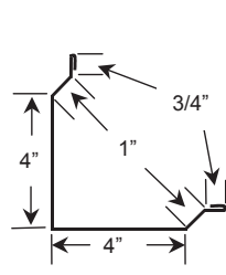
15. Outside Corner
