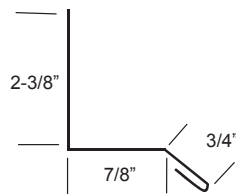
6. Drip Cap
