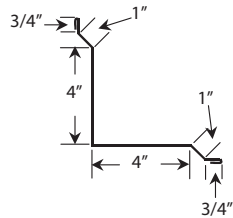
16. Inside Corner
