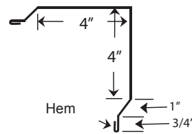
9. Gable Trim
