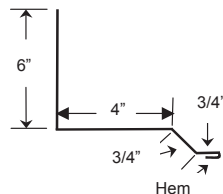
8. Sidewall Flashing
