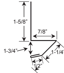
3. Rat Guard
